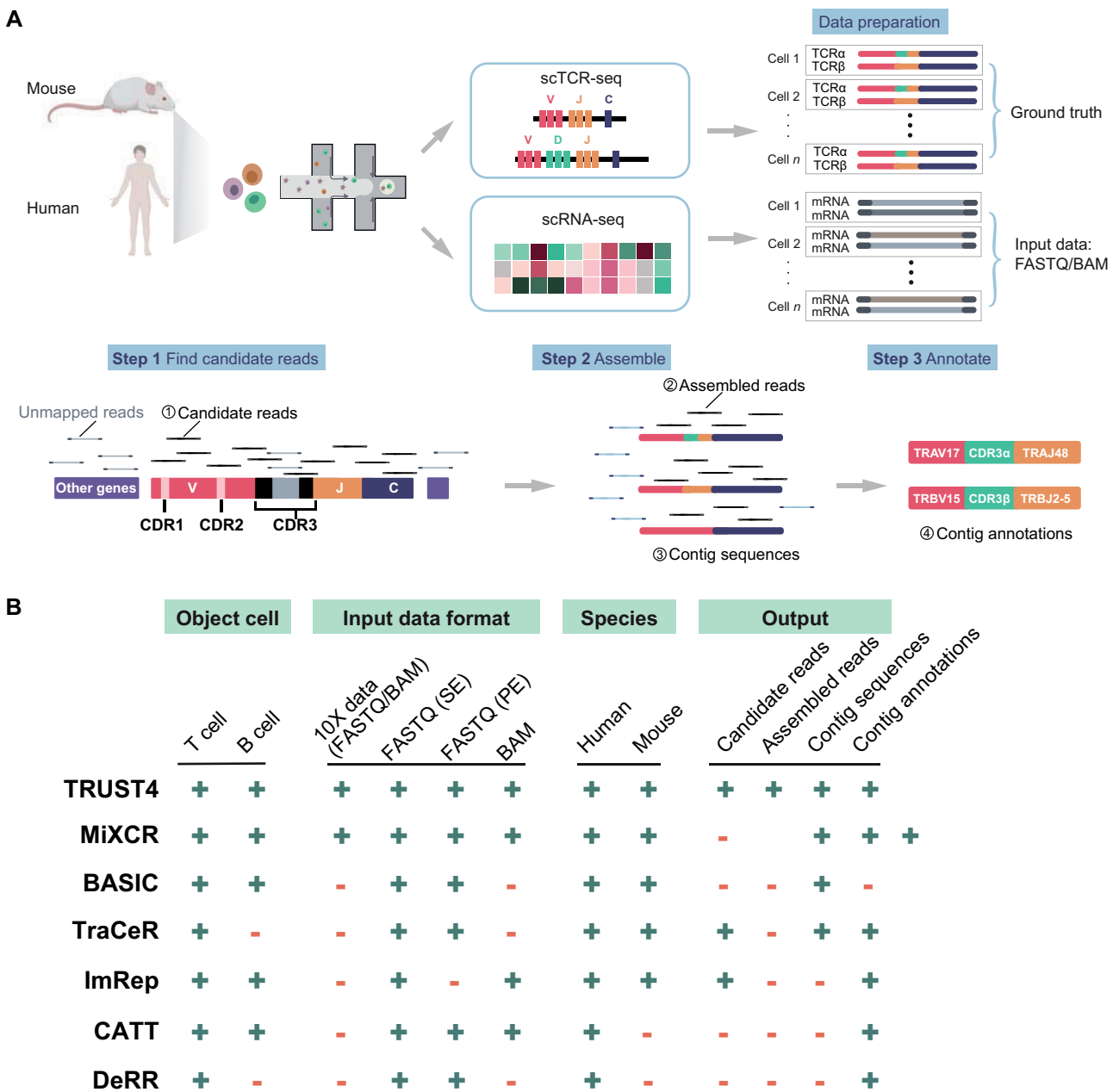
Figure 1 A benchmark framework for TCR construction methods using real scRNA-seq data
