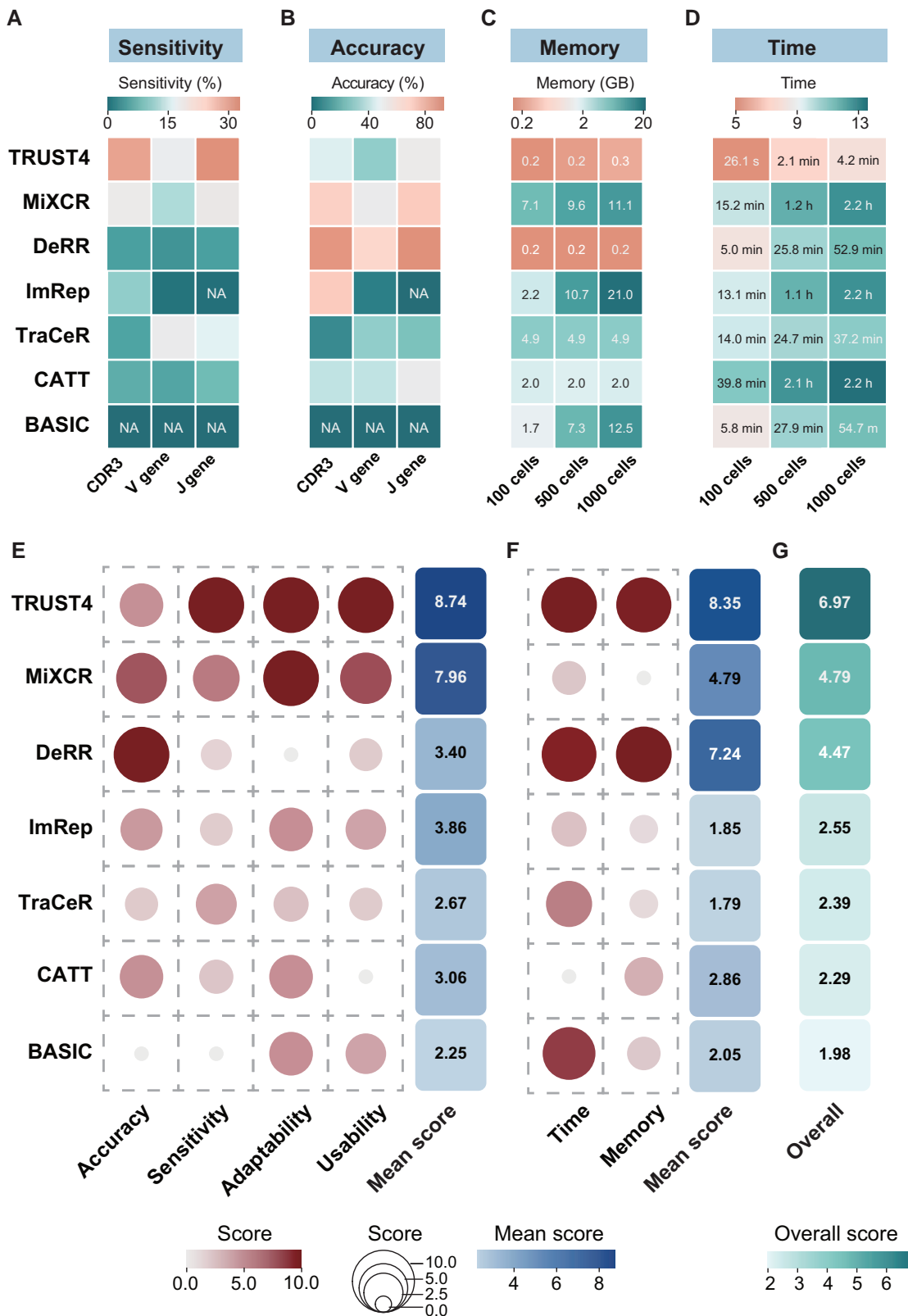
Figure 6 Comprehensive scoring and ranking for evaluating method performance
