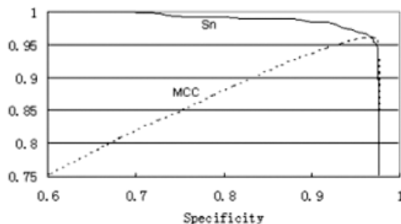
Fig. 2 The results of discriminating 653 human GPCRs from 10,845 non-GPCRs.
