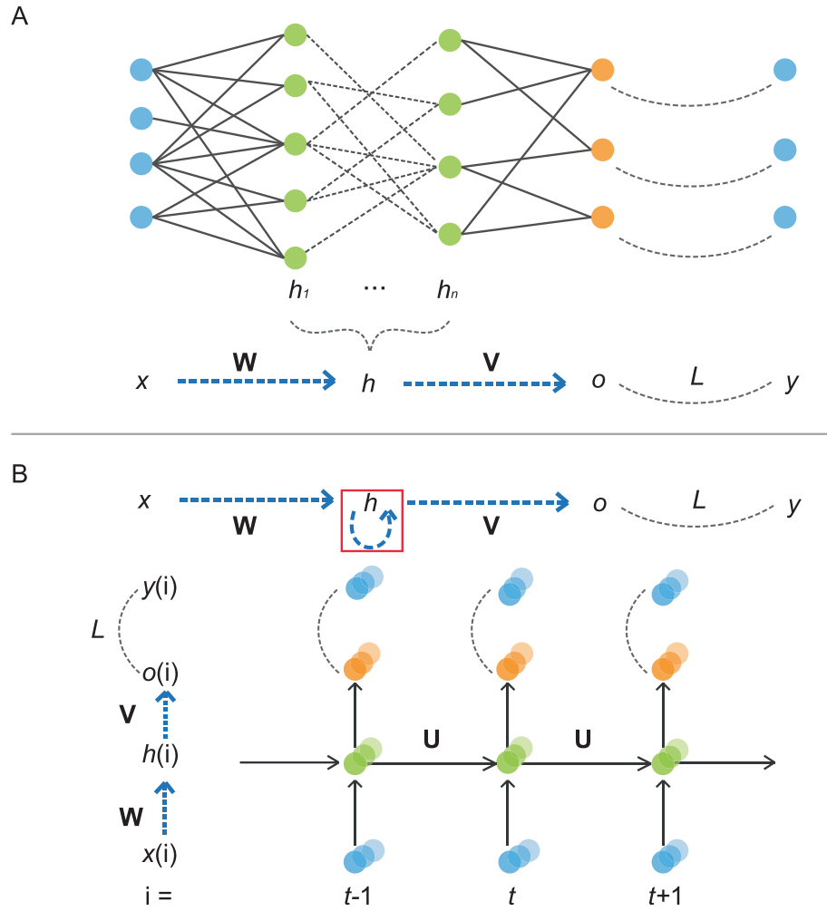
Figure 3 Illustration of recurrent neural network
