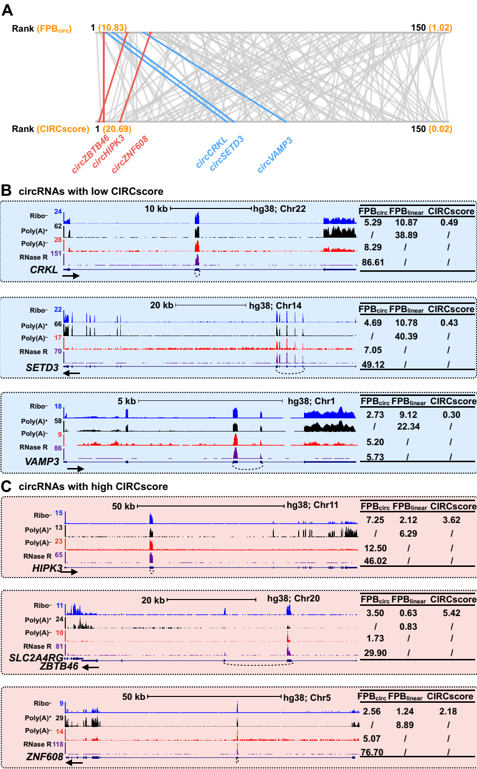
Figure 4 Difference of circRNA quantification by FPB and CIRCscore A. Difference in circRNA quantitation by FPB circ or CIRCscore in PA1 cells. About 150 circRNAs with FPB circ ≥ 1 were identified in PA1 cells from published ribo - RNA-seq (GEO: GSE73325 and GEO: GSE75733) [16,22]. Some circRNAs with high FPB circ values have high CIRCscore values due to the low background of cognate linear RNA expression (in red), while some others have low CIRCscore values due to the high background of cognate linear RNA expression (in blue). B. Three highly-expressed circRNAs, circCRKL , circSETD3 , and circVAMP3 , are co-expressed with their cognate linear RNAs at high levels, indicated by relatively low CIRCscores. The arcs represent the positions of circRNAs. C. Three highly-expressed circRNAs, circHIPK3 , circZBTB46 , and circZNF608 are co-expressed with their cognate linear RNAs at low levels, indicated by relatively high CIRCscores. The arcs represent the positions of circRNAs. Gene SLC2A4RG is presented in the figure, since it partially overlaps with the circRNA host gene ZBTB46 .
