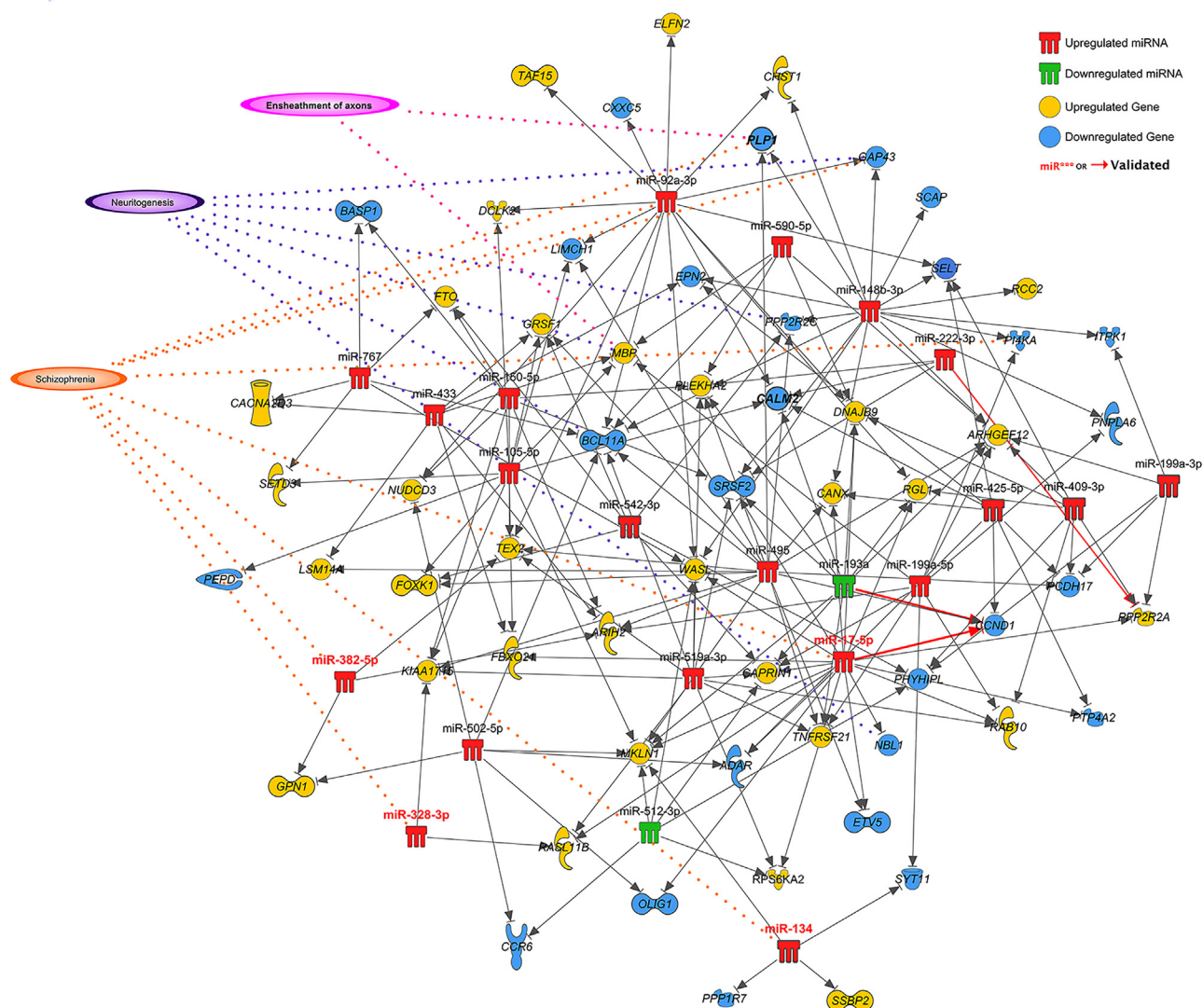
Figure 3 miRNA–gene regulatory interaction network involving miRNAs and genes dysregulated in DLPFC
