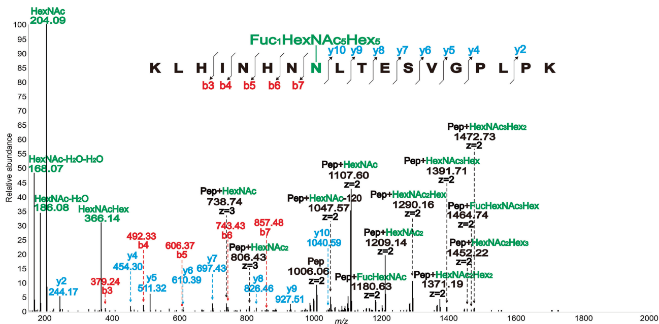
Figure 4 Annotated ESI MS2 spectrum showing N-glycosylation on the N8 in the peptide KLHINHNLTESVGPLPK
