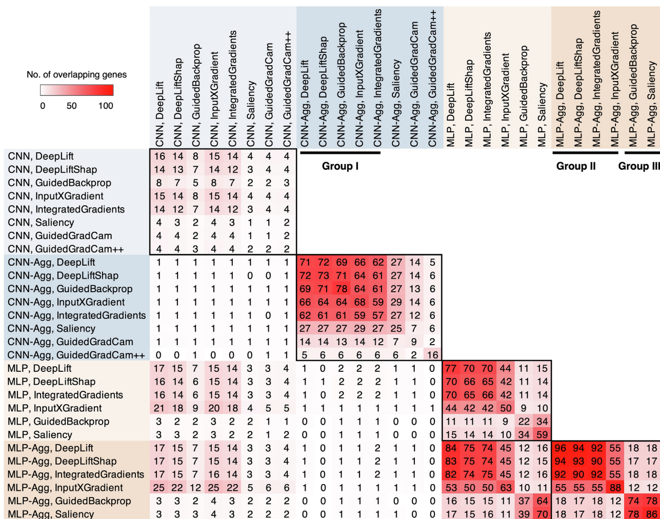
Figure 3 Overlap of the top 100 contributing genes across explainers with and without model aggregation
