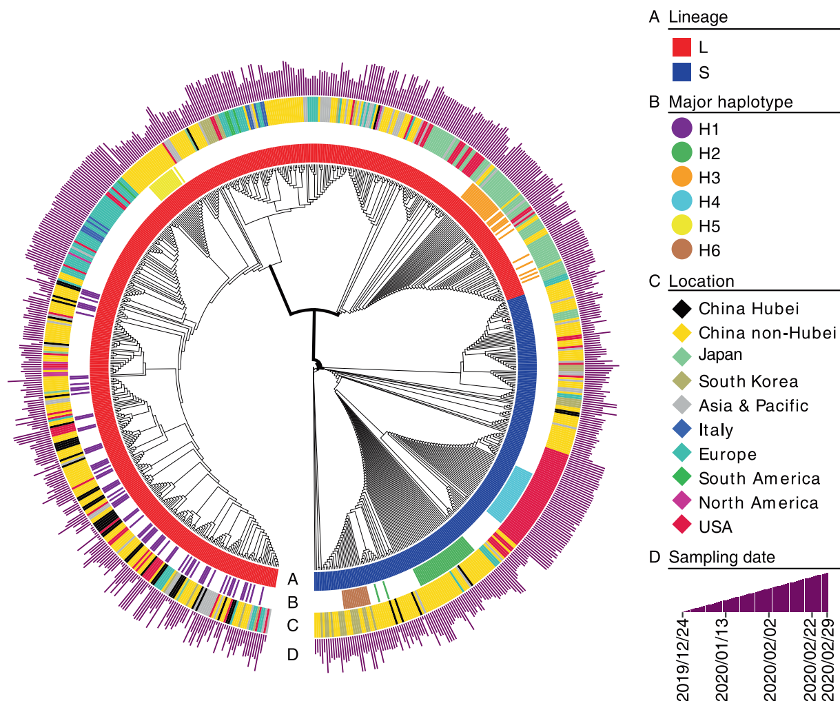
Figure 1 Neighbor-joining phylogeny of 756 SARS-CoV-2 sequences collected before Mar 1, 2020 and their sampling dates and locations. The 756 SARS-CoV-2 sequences were retrieved from 2019nCoV-R and GISAID. A. Two lineages (L and S lineages). B. Six major haplotypes with sequence count > 10 (H1–H6). C. Sampling locations (China and other countries or regions). D. Sampling date (Dec 24, 2019 to Feb 29, 2020). Samples are color coded. 2019nCoV-R, 2019 Novel Coronavirus Resource; GISAID, Global Initiative on Sharing All Influenza Data.
