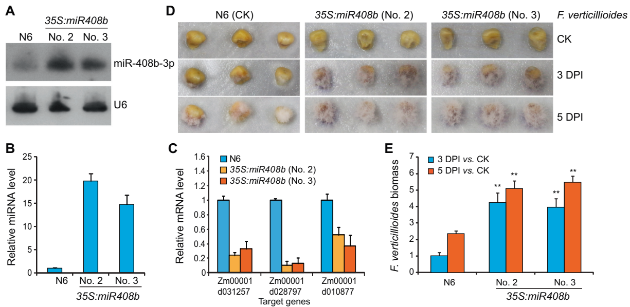
Figure 7 miR408b affects the degree of resistance to F. verticillioides of the susceptible maize genotype RNA blot analysis
