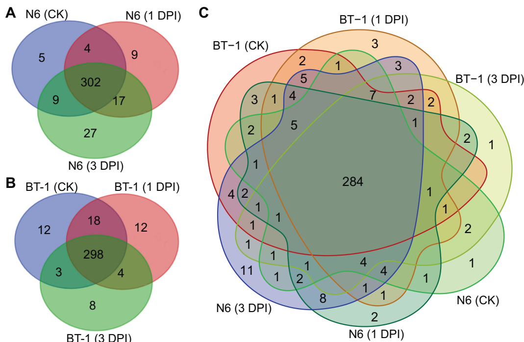
Figure 2 Venn diagram showing miRNAs detected by deep sequencing of maize kernels exposed or not to F. verticillioides
