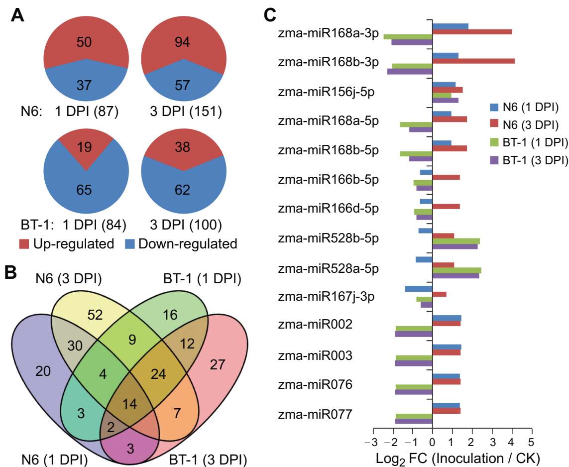
Figure 3 F. verticilloides -responsive miRNAs in the susceptible and resistant genotypes
