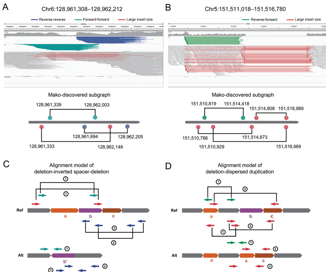
Figure 5 Two representative CSV subgraphs identified by Mako
